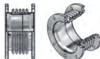
PRFA expansion joint with fixed flanges
