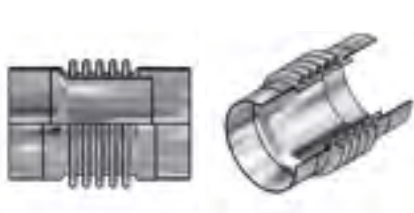
PRRA expansion joint with welding ends
